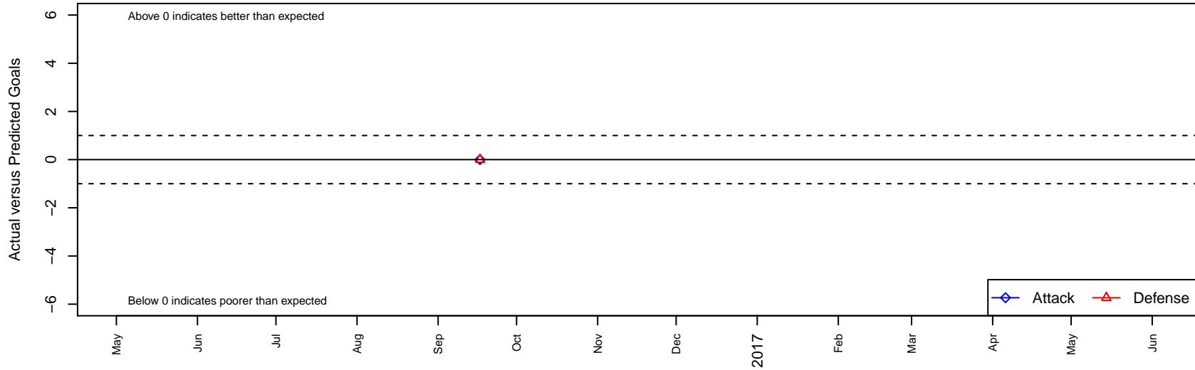
Diablo FC NPL B03 Dots are actual minus expected GF (blue circles) and GA (red triangles). Blue line is smoothed change in attack strength. Red is smoothed change in defense strength.
